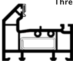
56MM PVC-U THRESHOLD (BEVELLED)
